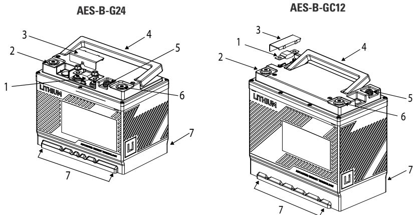
Figure 2. Lithium BLUE Battery Components
