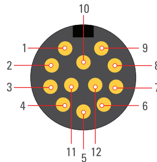
Circular 12 PIN
