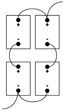
Series/Parallel Connection
