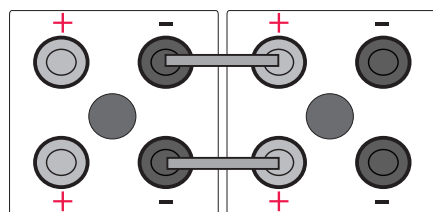
2 Volt 4 Pole (Sliding) Battery Cells
