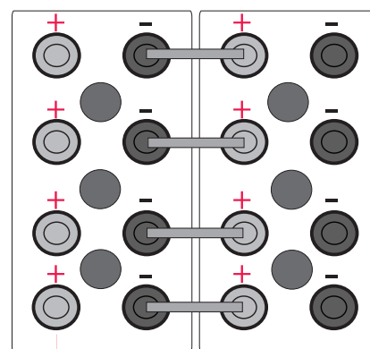
2 Volt 8 Pole (Sliding) Battery Cells
