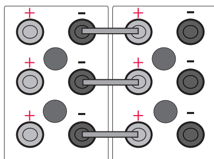
2 Volt 6 Pole (Sliding) Battery Cells
