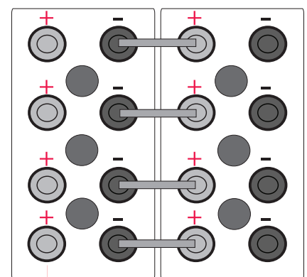
2 Volt 8 Pole (Sliding) Battery Cells
